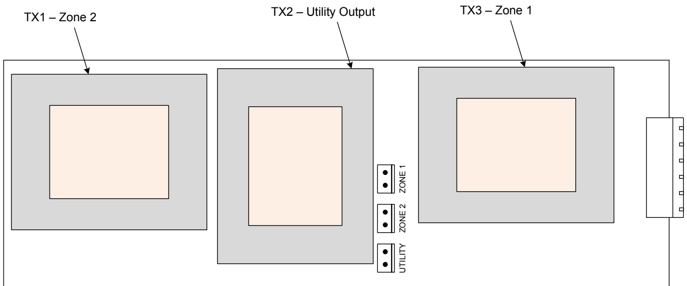
CXL-3120 transformer module PCB assembly
