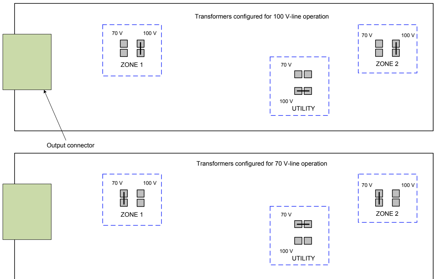
SOLDER SIDE OF PCB, SHOWING APPROX. LOCATIONS OF WIRE LINKS
