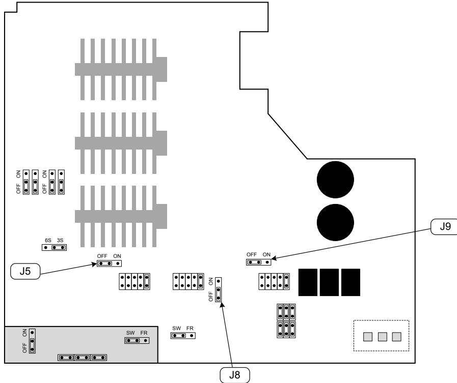
36-50 Jumper locations for Step 5.
